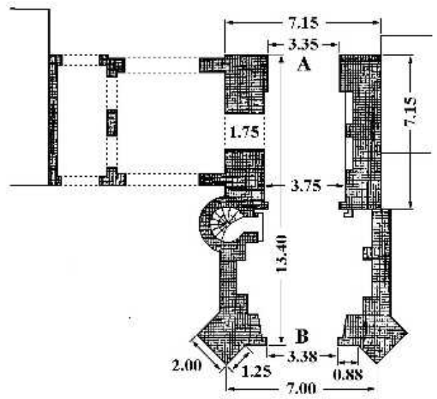
Grundriß Erdgeschoß
