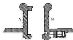
Grundriß Erdgeschoß
